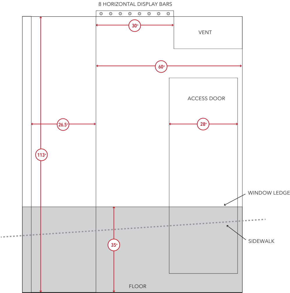
ELEVATION (STRAIGHT-ON VIEW FROM THE STREET) (MEASUREMENTS APPROXIMATE)
